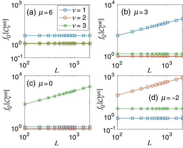
FIG. 2. Dual QFI density f_Q[\mathcal{O}_\nu^{(\text{st})}, |\mathcal{G}\rangle] of the ground state |\mathcal{G}\rangle versus L for the extended Kitaev chain with N_f = 3 and nonzero parameters ( J_1^\pm = 1 , J_2^\pm = 2 , J_3^\pm = 2 ) in different topological phases. (a) For \mu = 6 , the winding number \nu = 0 . (b) For \mu = 3 , \nu = 1 , and the fitting nontrivial scaling topological index \lambda_1^{(\text{st})} = 0.9965 . (c) For \mu = 0 , \nu = 3 , and \lambda_3^{(\text{st})} = 1.0047 . (d) For \mu = -2 , \nu = 2 , and \lambda_2^{(\text{st})} = 0.9957 .
