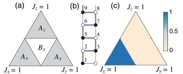
FIG. 4. (a) The phase diagram of the Kitaev honeycomb model on the J_x + J_y + J_z = 1 plane. In the region J_x \leq J_y + J_z , J_y \leq J_z + J_x , and J_z \leq J_x + J_y , there is a gapless phase B with non-Abelian excitations, and in other regions, there are three gapped phases A_{x,y,z} with Abelian anyon excitations. (b) A single-chain representation of the two-leg spin ladder of the Kitaev model. (c) The scaling topological index \lambda_x^{(\text{st})} of the dual QFI density f_Q[\mathcal{O}_x^{(\text{st})}, |\mathcal{G}\rangle] for different values of J_{x,y,z} versus system size 2L up to 400.
