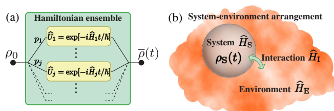
FIG. 1. (a) Schematic illustration showing the averaged state \bar{\rho}(t) resulting from the Hamiltonian ensemble \{(p_j, \hat{H}_j)\} . The averaged state, in general, follows incoherent dynamics; i.e., similar to open quantum systems, its time evolution cannot be accurately captured by the von Neumann equation alone. (b) If a quantum system interacts with a bath, their interaction will, in general, correlate them. As we show, the nature of these correlations, i.e., classical or quantum, is intimately connected to the (im)possibility to simulate the dynamics of the open system with a Hamiltonian ensemble.
