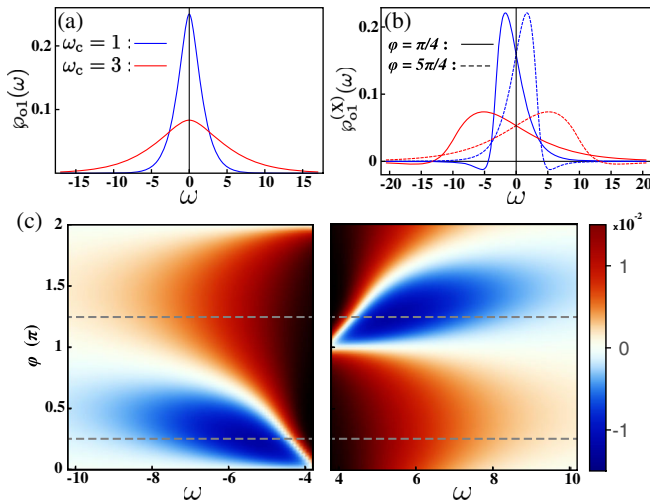
FIG. 2. (a) Legitimate probability distributions \varphi_{o1}(\omega) for the conventional spin-boson model. (b) Distributions \varphi_{o1}^{(X)}(\omega) for the extended model, violating positivity. (c) The landscape of negative contributions to \varphi_{o1}^{(X)}(\omega) against \omega and \varphi for \omega_c = 1 . The gray dashed lines denote the positions in (b).
