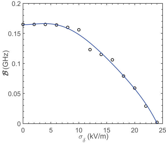
FIG. 3. The bandwidth of the negative refraction \mathcal{B} vs \sigma_\delta for \bar{\delta} = 1 MV/m, n_0 = 0.5 ppm, B = 800 G, and T = 20 K. Here, we assume the ensemble of NV centers are exposed to random strain fields of normal distribution with mean \bar{\delta} and standard deviation \sigma_\delta .
