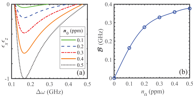
FIG. 4. The dependence of negative refraction on the density of NV centers n_0 . (a) The product of two components of permittivity tensor \epsilon_x\epsilon_z vs detuning \Delta\omega = \omega - \Delta_{fi} ; (b) The bandwidth \mathcal{B} vs n_0 . The intensity of magnetic field is B = 800 G. Other parameters are d_x = d_y = 11 D [75], \gamma = 50 MHz at T = 20 K [74], \epsilon_D = 5.7 [76], and \mu_D = 1 - 2.1 \times 10^{-5} [77].
