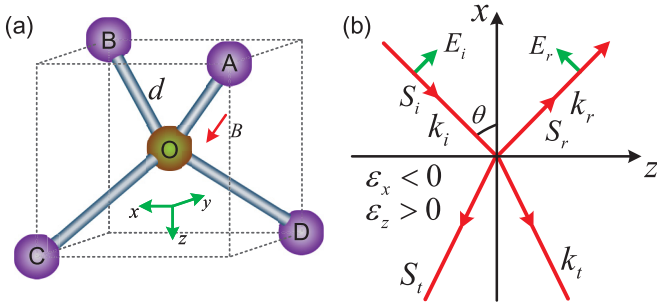
FIG. 1. (a) Four possible orientations of NV centers in diamond [29,68]: \vec{r}_{OA} = (-1, -1, -1)/\sqrt{3} , \vec{r}_{OB} = (1, 1, -1)/\sqrt{3} , \vec{r}_{OC} = (1, -1, 1)/\sqrt{3} , \vec{r}_{OD} = (-1, 1, 1)/\sqrt{3} . d = 154 pm is the length of carbon bond. The angle between any pair of the above four orientations is identically \alpha = 109^\circ 28' . The magnetic field \vec{B} is along -\vec{r}_{OA} . (b) Negative refraction for hyperbolic dispersion with \epsilon_x < 0 and \epsilon_z > 0 . The TM mode is incident on the yz interface with electric field \vec{E}_i , wave vector \vec{k}_i , and Poynting vector \vec{S}_i . The angle between the normal ( x axis) and the incident field is \theta . It is reflected with electric field \vec{E}_r , wave vector \vec{k}_r , and Poynting vector \vec{S}_r . The Poynting and wave vector of the transmitted wave are, respectively, \vec{S}_t and \vec{k}_t .
