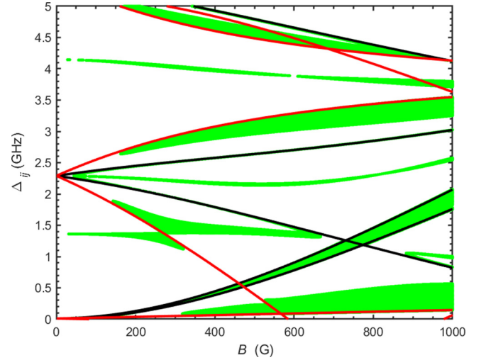
FIG. 2. The negative refraction (green shadows) versus \Delta_{ij} = E_i^e - E_j^g - 1.945 eV and B when the magnetic field is applied along the direction of (1,1,1). The transition frequencies are identical and denoted by black curves for the NV centers of orientations along \vec{r}_{OB} , \vec{r}_{OC} , \vec{r}_{OD} in Fig. 1(a) due to the special choice of \vec{B} . The transition frequencies for the NV centers of orientation along \vec{r}_{OA} are different and denoted by red curves. The density of NV centers is n_0 = 0.5 ppm and the decay rate of the excited state is \gamma = 50 MHz at T = 20 K [74].
