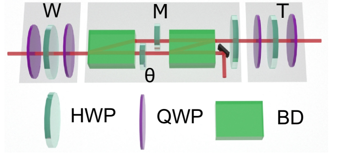
FIG. 8. Optical simulation of the nonunitary time-evolution operator.
