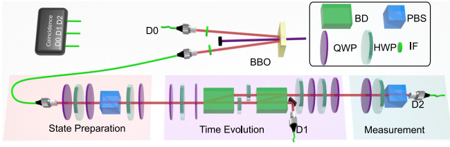
FIG. 1. Sketch of the experiment. The idler photon is detected by D0 for coincidence counting. The signal photon enters the setup, which consists of three parts: state preparation, time evolution, and state measurement. The photon loss is collected by D1. BBO: \beta -barium-borate; PBS: polarization beam splitter; BD: beam displacer; HWP: half-wave plate; QWP: quarter-wave plate; IF: interference filter; D0, D1, and D2 are single photon detectors.
