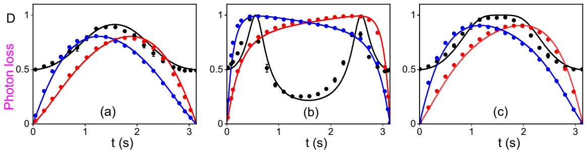
FIG. 3. Time evolution of the states when \epsilon = \pi/6 with (a) s = 1.1 , (b) s = 3 , and (c) s = 1.225 . The black lines are the dynamics of the trace distance D between the time-evolved states U_{\mathcal{PT}}|\psi_1\rangle and U_{\mathcal{PT}}|\psi_2\rangle . The red (blue) lines indicate the dissipations of |\psi_1\rangle ( |\psi_2\rangle ) into the environment. Dots with error bars are the experimental data while lines are the theoretical simulations.
