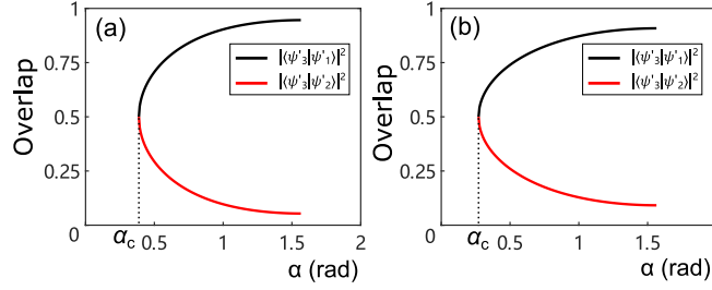
FIG. 9. Theoretical overlaps between the normalized time-evolved states, |\langle\psi'_3|\psi'_1\rangle|^2 and |\langle\psi'_3|\psi'_2\rangle|^2 , with different \alpha for (a) \beta = \pi/3 and (b) \beta = \pi/2 in our experiment.
