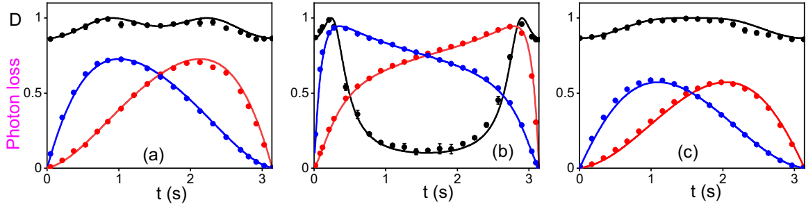
FIG. 2. Time evolution of the states when \epsilon = \pi/3 with (a) s = 1.1 , (b) s = 3 , and (c) s = 1.038 . The black lines are the dynamics of the trace distance D between the time-evolved states U_{\mathcal{PT}}|\psi_1\rangle and U_{\mathcal{PT}}|\psi_2\rangle . The red (blue) lines indicate the dissipations of |\psi_1\rangle ( |\psi_2\rangle ) into the environment. Dots with error bars are the experimental data while lines are the theoretical simulations.
