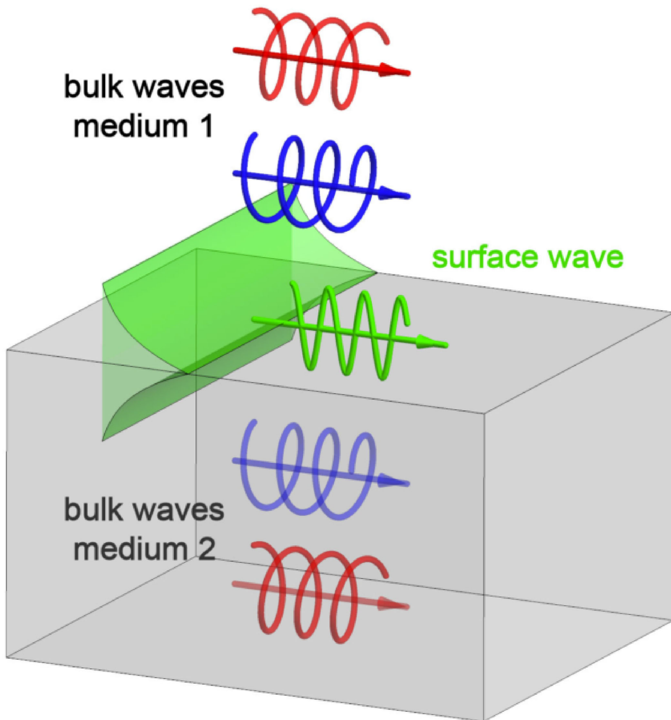
An interface between media with different helicities (red and blue curly arrows) supports zero-helicity linearly polarized surface modes (green arrow). Credit: Konstantin Bliokh
