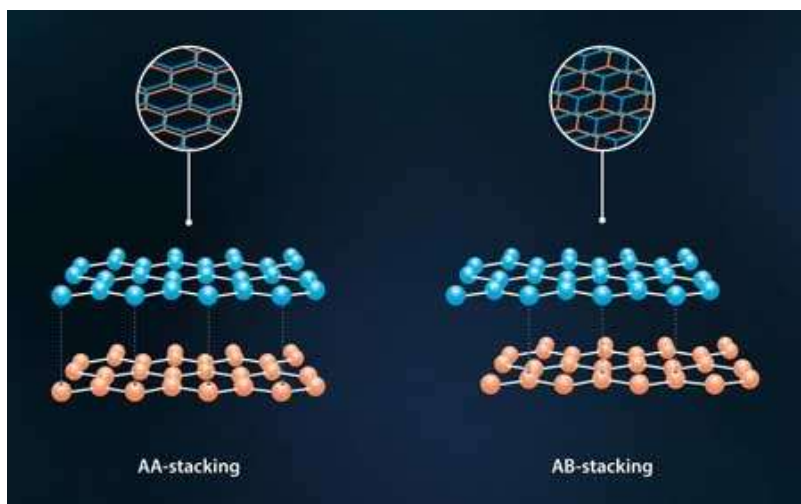
Fig. 1. Two types of bigraphene: AA-stacked bilayer graphene where each atom in the upper sheet sits exactly on top of an atom in the lower sheet and AB-stacked bilayer graphene where only half of the atoms in the upper sheet lie over another atom, whereas the other half lie over the center of a hexagon formed by the atoms in the lower sheet.
