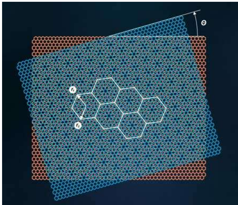
Fig. 2. The third type of bigraphene known as twisted bilayer graphene. The white hexagons mark the boundaries of superlattice cells (moiré pattern cells).
