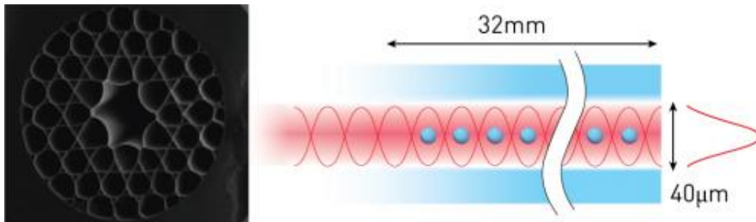
Figure 1: A hollow-core optical fiber supports a kagome lattice (left) that can confine atoms in the central channel in a regular coherent state (right). Credit: Reproduced from Ref. 1 and licensed under CC BY-NC-ND 4.0 © 2014 S. Okaba et al.
