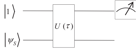
FIG. 1. Quantum circuit for obtaining the energy spectrum of a physical system. The first input register represents a probe qubit, and the second input register represents the system whose spectrum we are trying to obtain.
