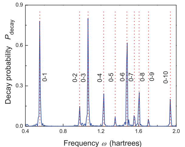
FIG. 3. (Color online) Same as in Fig. 2, except the operator A is set as shown in Eq. (6).
