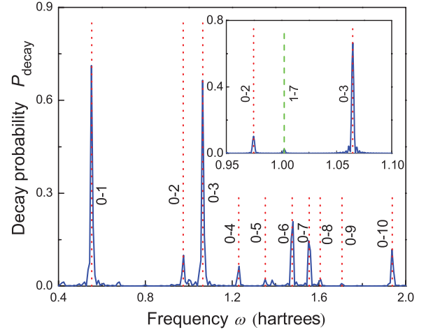
FIG. 2. (Color online) Transition frequency spectrum between the ground state, |\varphi_0\rangle , and the first ten excited states ( |\varphi_i\rangle, i = 1, 2, \dots, 10 ) of the water molecule. The blue solid curve represents the decay probability of the probe qubit at different frequencies with the coupling coefficient in Eq. (1) c = 0.005 and the evolution time \tau = 500 , and the operator A as shown in Eq. (5). The red dotted vertical lines represent the known transition frequencies between the ground state and the first ten excited states of the water molecule. In the inset, the second and the third transition frequencies shown in blue were obtained using c = 10^{-3} and \tau = 2500 . The green vertical dashed line represents the known transition frequency (1-7) between the first and the seventh excited states.
