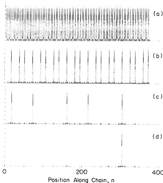
FIG. 3. Probability density, P_n , vs site position, n , along the chain. In (a)–(d) the probability densities have contributions from the states belonging respectively to (a'), (b'), (c'), and (d'), where (a') denotes the central main cluster of states around E = 0 in Fig. 1(a), (b') the central subcluster of (a'), (c') the central subcluster of (b'), and (d') the central subcluster of (c').
