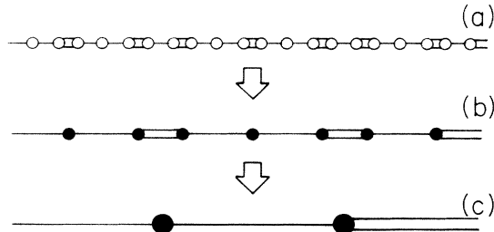
FIG. 4. Schematic representation of the decimation procedure favoring the bonding molecular states. The double (single) lines denote the strong (weak) effective bonds. The isolated atoms in (a) are eliminated, producing the renormalized chain in (b). Eliminating the isolated atoms again obtain the renormalized chain in (c).
