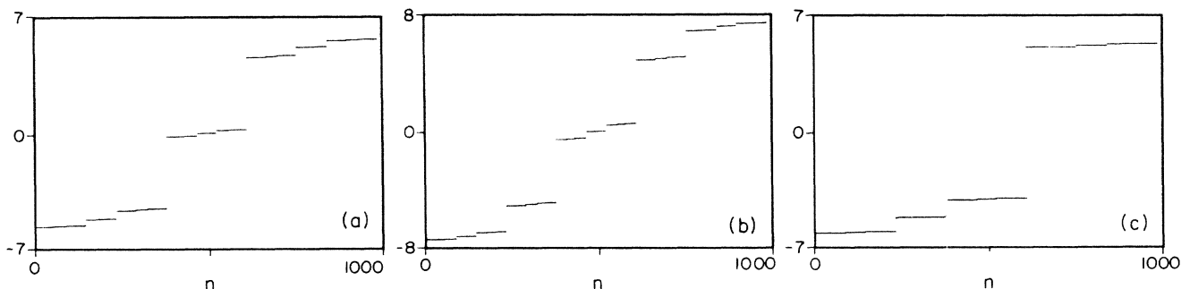
FIG. 1. Energy spectrum of our model in the three cases, (A), (B), and (C), specified in the text. The eigenenergies are plotted from left to right in increasing order. The lattice has 987 sites and fixed-end boundary conditions. (a) Case (A), with T_w = 1 and T_s = 5 ; (b) case (B), with T_w = 1 and T_s = 5 ; (c) case (C), with T = 1 , V_1 = -5 , and V_2 = 5 .
