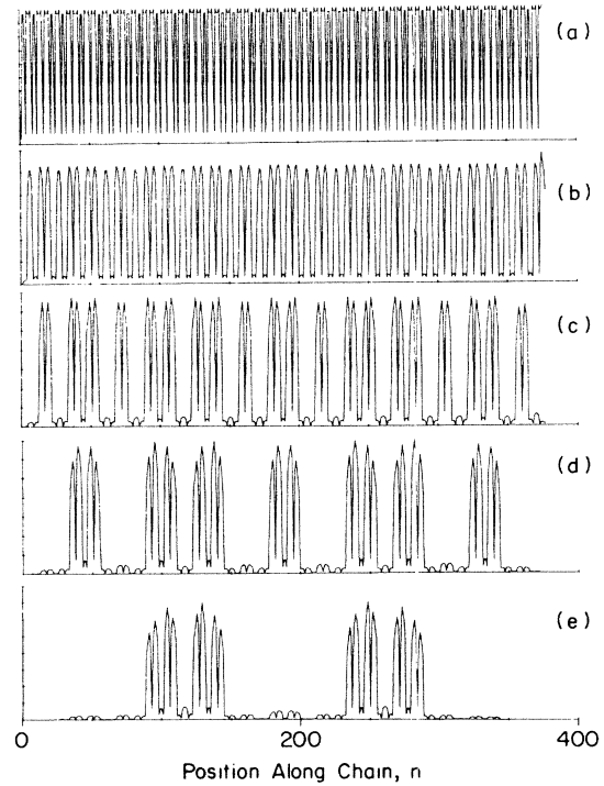
FIG. 5. Probability density, P_n , vs site position, n , along the chain. In (a)–(e) the probability densities have contributions from the states belonging to (a''), . . . , (e'') respectively, where (a'') denotes the top main cluster of Fig. 1(a), (b'') the top subcluster of (a''), (c'') the top subcluster of (b''), and so on.
