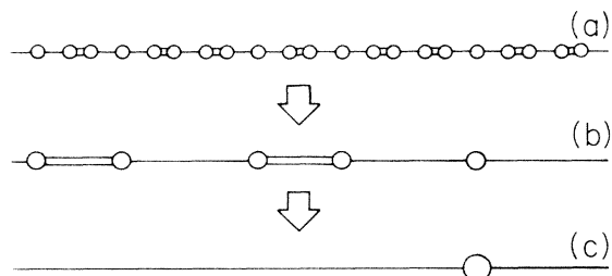
FIG. 2. Schematic representation of the decimation procedure favoring the atomic sites. The double (single) lines denote the strong (weak) effective bonds. The molecules in (a) are eliminated, producing the renormalized chain in (b). Eliminating the new molecules, we obtain the renormalized chain in (c).
