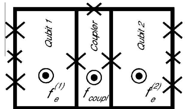
Fig. 1. Schematic diagram of two coupled flux qubits, each one with four Josephson junctions. These qubits can be coupled [24] via the central coupler loop allowing to change the magnitude and sign of the coupling constant g .
